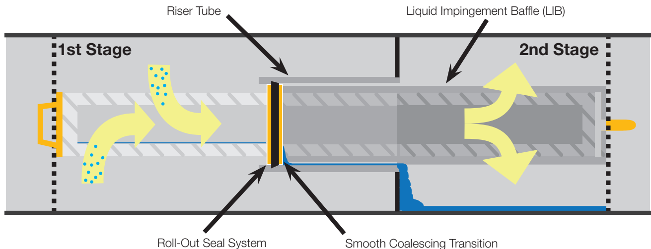
PGC2 CARTRIDGE OPERATION IN VESSEL
